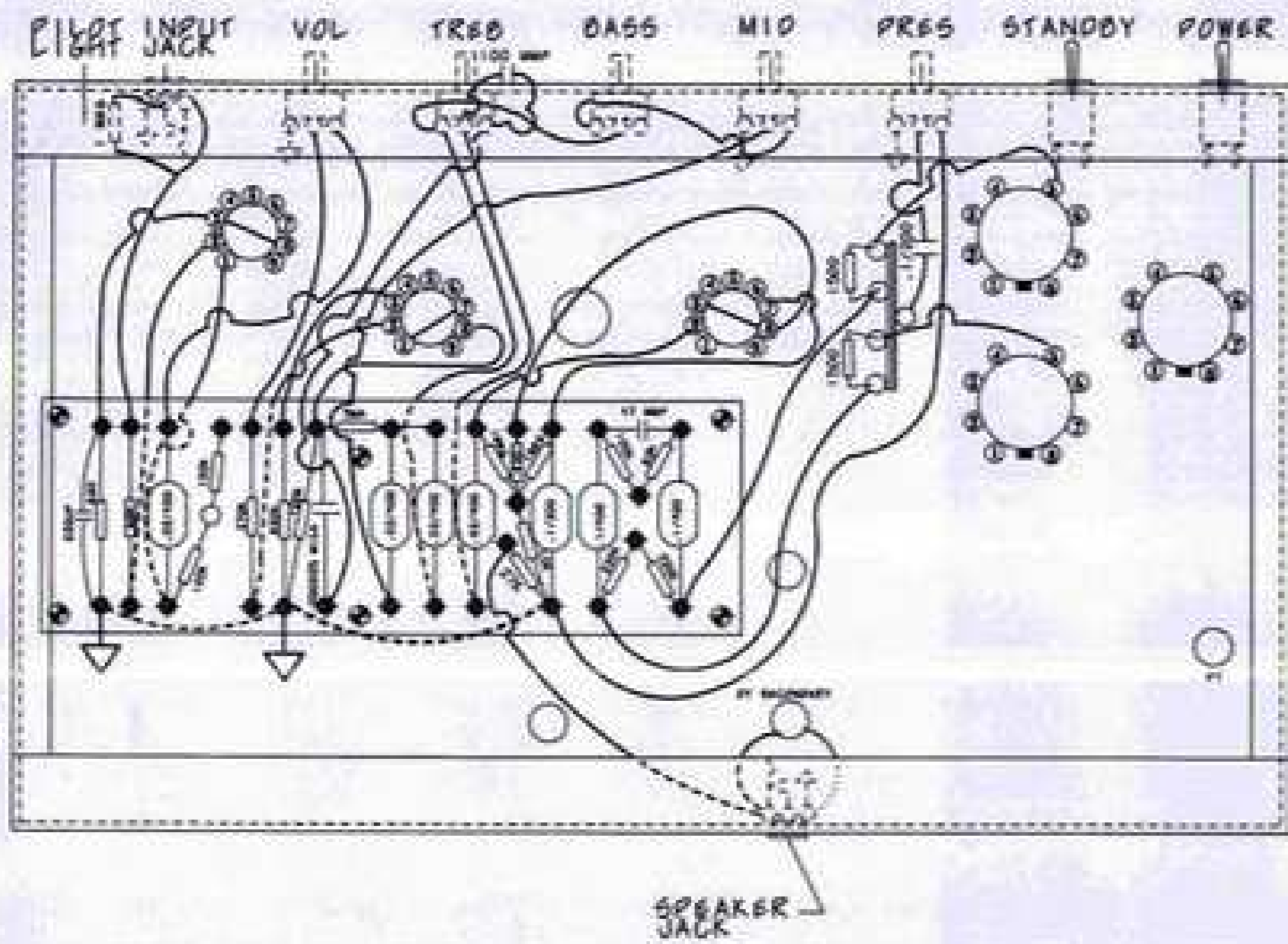
DUKANE 1U460A CONVERSION TO 5F6A SIGNAL GRID PATH
